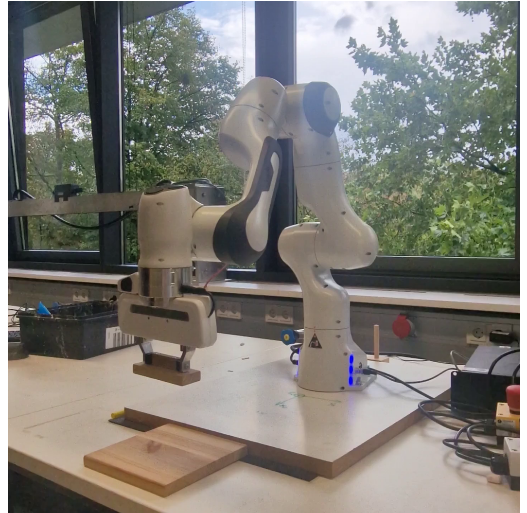
Null-space demonstration 2
